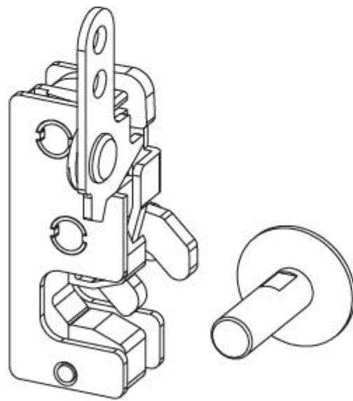
Unlocked position
